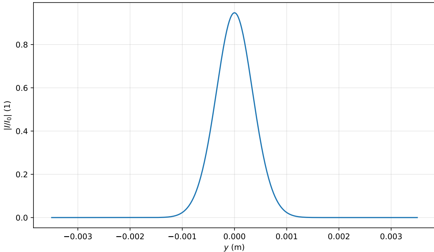
Intensity profile I(x=0, y, z=0.716)/I_0 , P_{in}=0.2P_{cr} , artificial time
